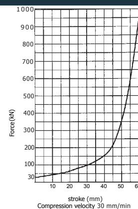
STANDARD DRAWGEAR SPRING, COMPLIANT WITH EN 15566:2016
