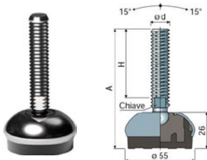
PIEDE SNODATO D. 55 Art. 485 Articulated Foot D.55 Art. 485
