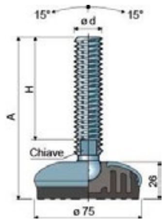
PIEDE SNODATO D.75 Art. 499 Articulated Foot D.75 Art. 499
