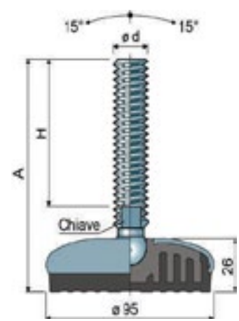
PIEDE SNODATO D.95 Art. 494 Articulated Foot D.95 Art. 494
